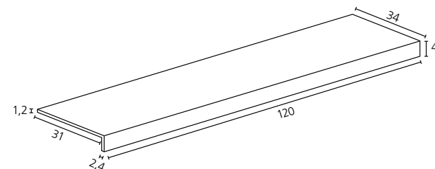
GRADINO PLUS** 34x120x4,5 cm RECT - 13 3 / 8 "x48x1 3 / 4 " SOFT ± 10 mm
