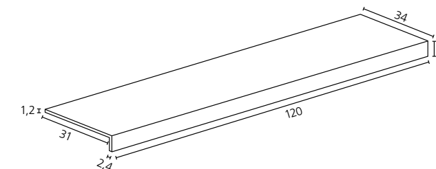
GRADINO PLUS** 34x120x4,5 cm RECT - 13 3 / 8 "x48x1 3 / 4 " LUX* ± 10 mm
